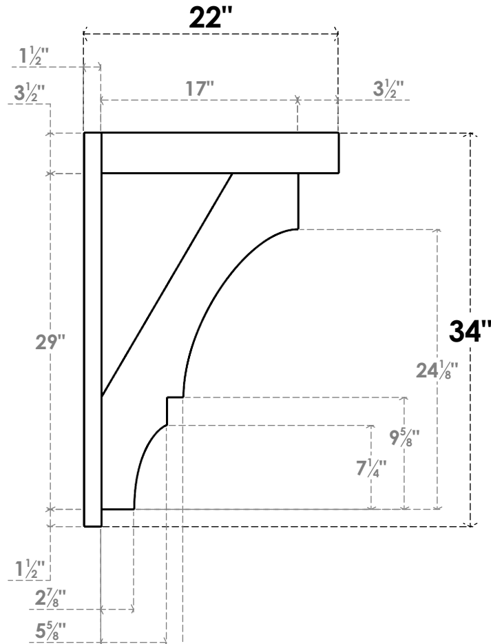
SIDE PROFILE
